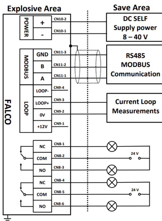
Figure showing typical connector wiring diagram.
