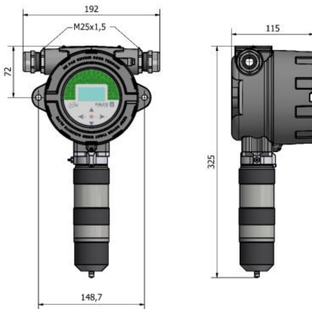
Figure 2 Dimensioned Drawing of Falco 2.2 with Pump
